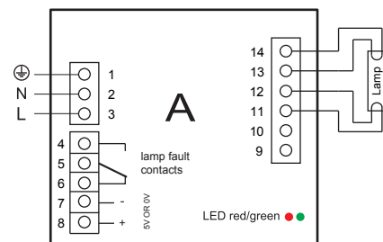
Wiring Diagram
